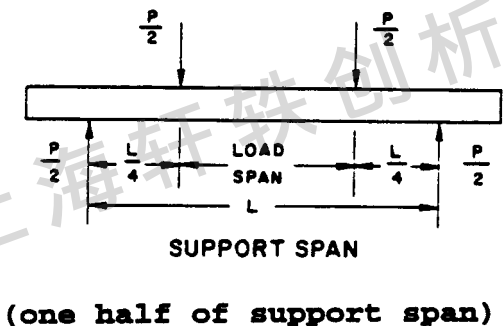
FIG. 1 Loading Diagram
